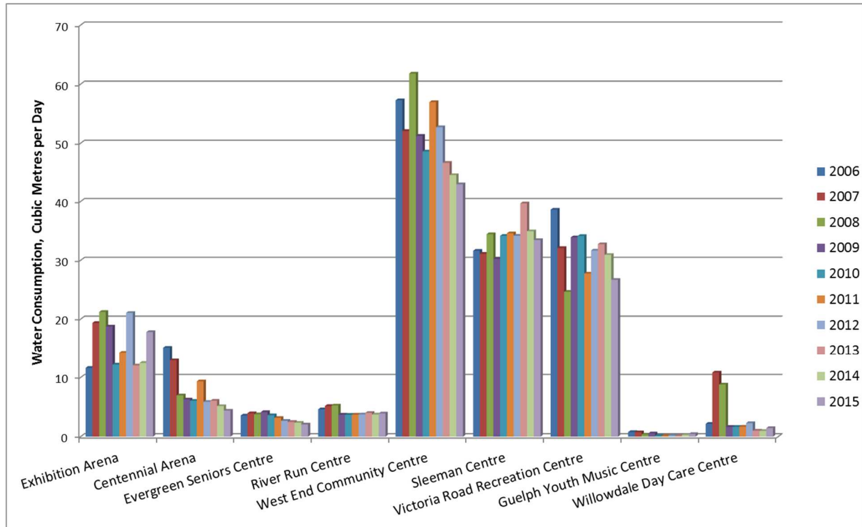
Figure 1: City of Guelph Recreation Facilities Average Daily Water Consumption (2006-2015)
