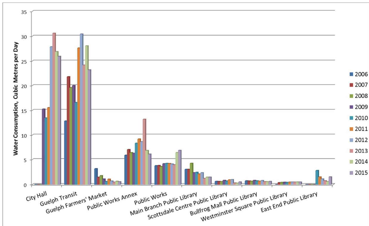
Figure 2: City of Guelph Public Facilities Average Daily Water Consumption (2006-2015)
