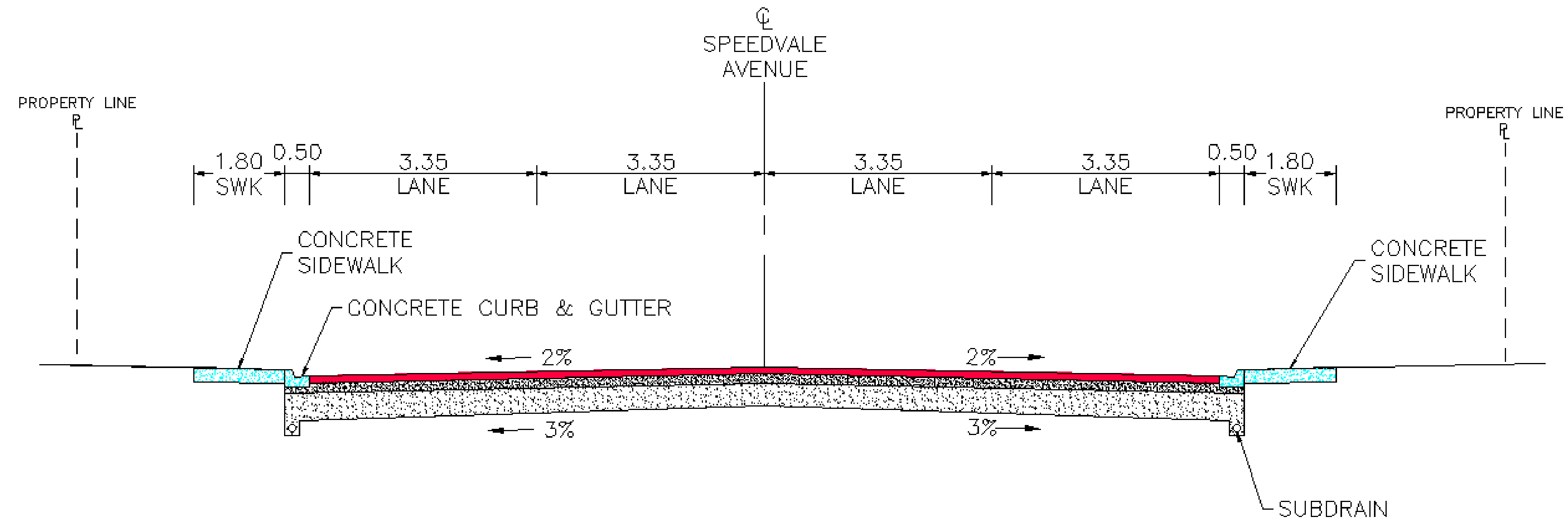
TYPICAL SECTION WITH SIDEWALK
