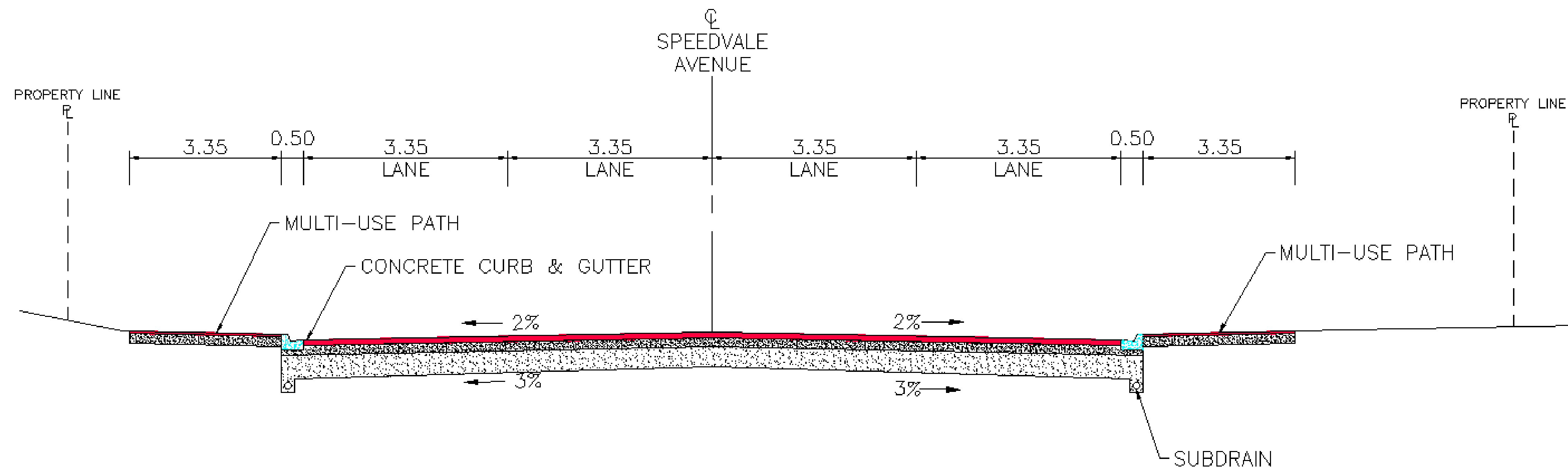
TYPICAL SECTION WITH MULTI-USE PATH
