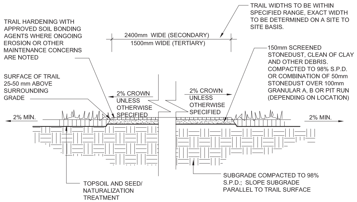
Fig. 5-5 Off-Road Trail Detail: Natural Area Buffer
