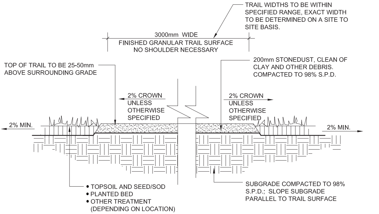
Fig. 5-3 Off-Road Trail Detail: Major City Wide Destination
