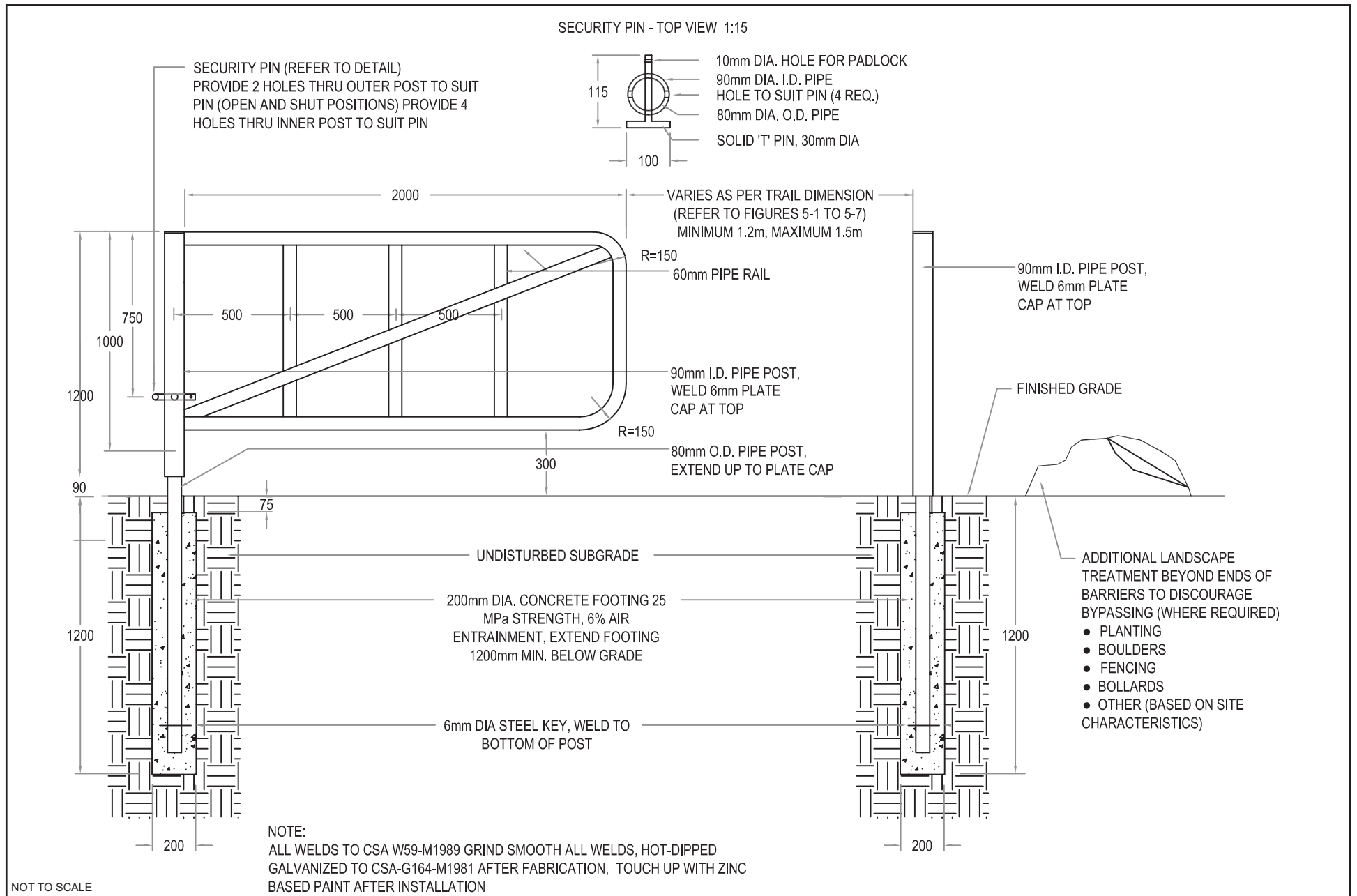
Fig. 5-12 Trail Access Barrier
