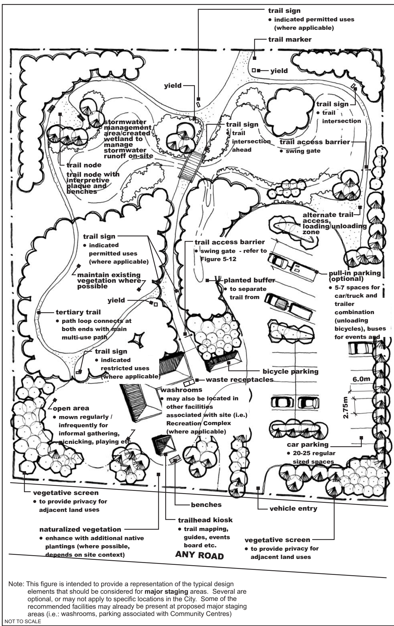
Fig. 5-11 Elements of a Typical Major Trailhead / Staging Area
