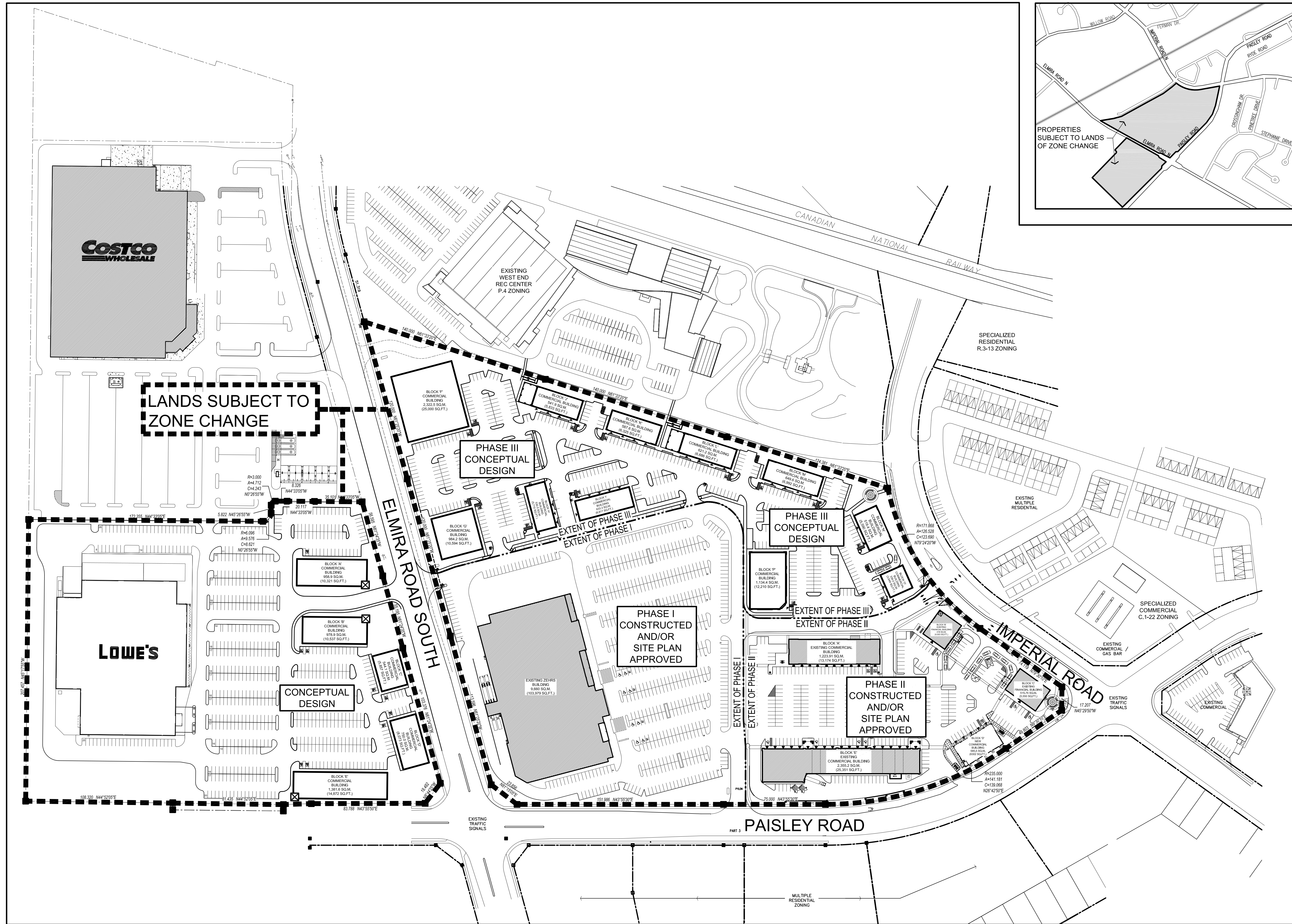
1 SITE PLAN scale: 1:1250
