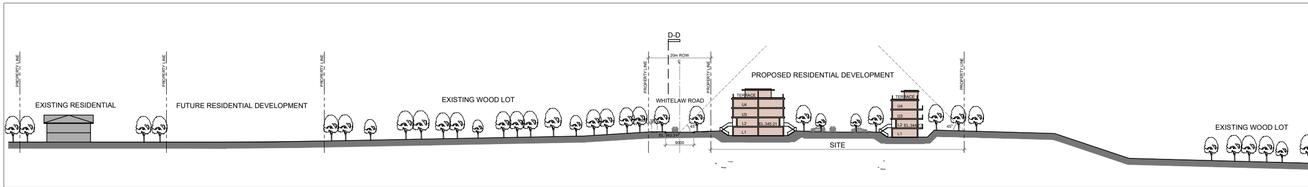
Site Section A-A East-West Looking South thru Proposed Stacked Townhouses
