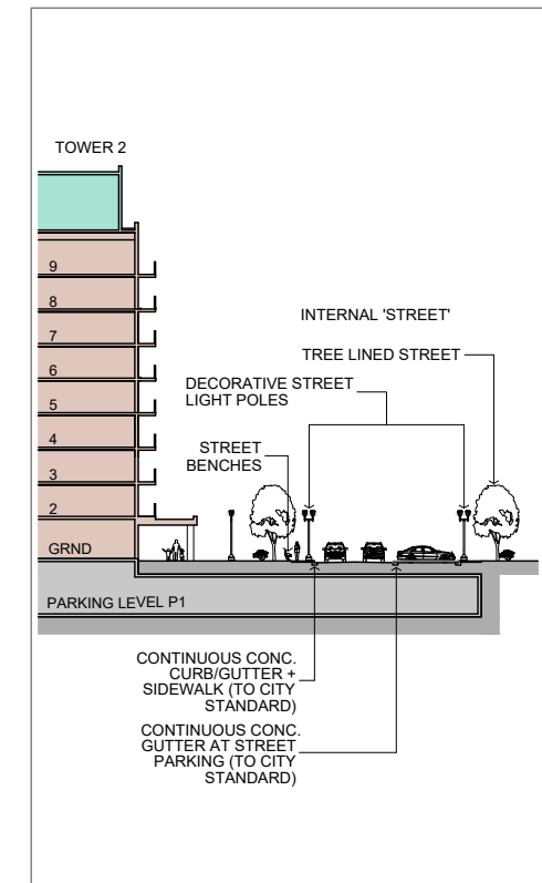
Internal Street Section (NTS)
