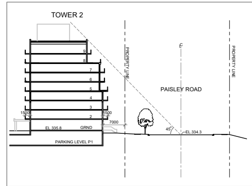
Site Section K-K North-South Looking West
