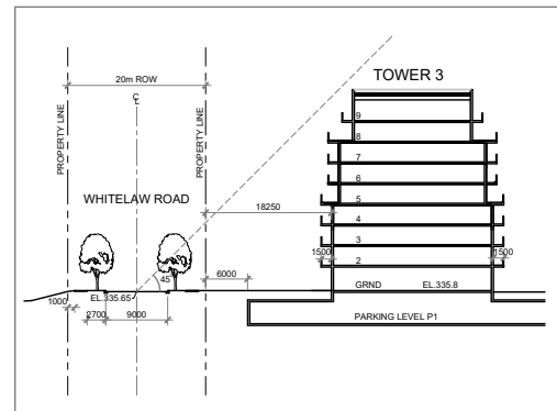
Site Section F-F East-West Looking South
