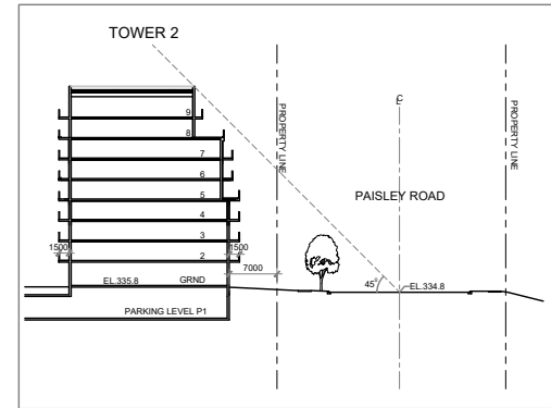
Site Section L-L North-South Looking West
