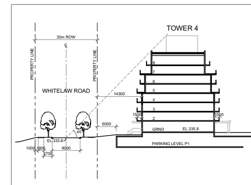
Site Section G-G East-West Looking South
