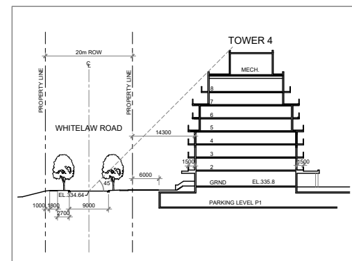
Site Section H-H East-West Looking South
