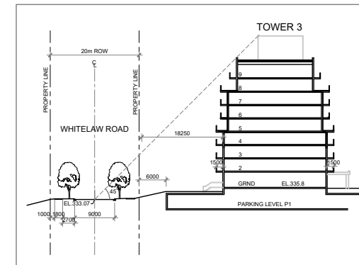
Site Section E-E East-West Looking South
