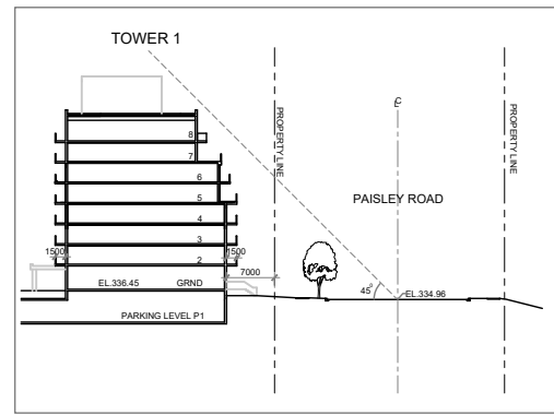
Site Section M-M North-South Looking West
