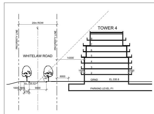
Site Section J-J East-West Looking South
