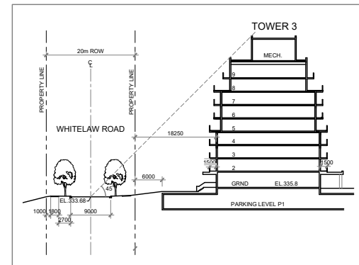
Site Section B-B East-West Looking South
