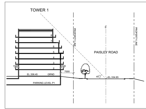
Site Section N-N North-South Looking West
