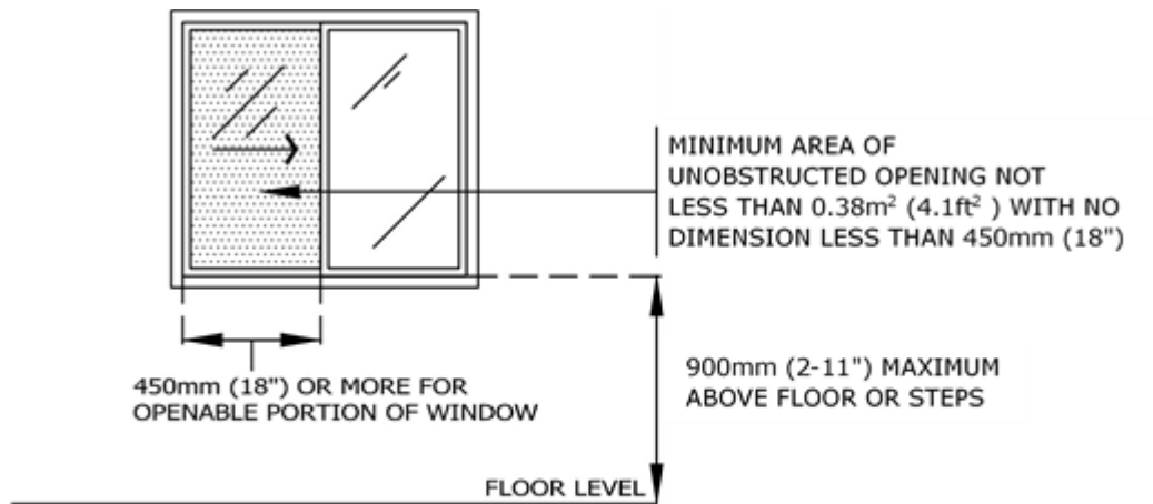
Image 1: Window providing additional means of escape (C136)
