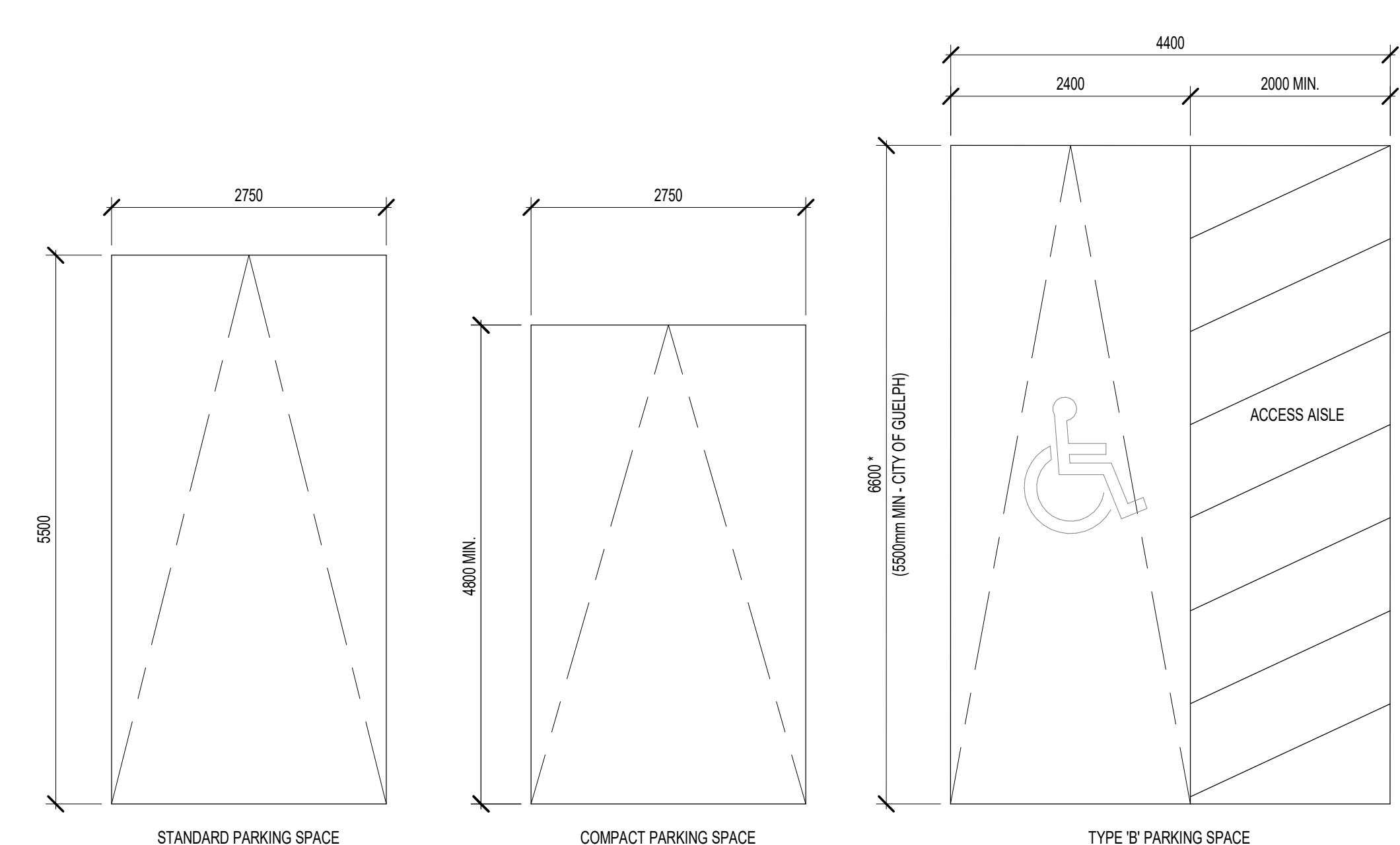
2 PARKING SPACE SCHEDULE A200 1:50
