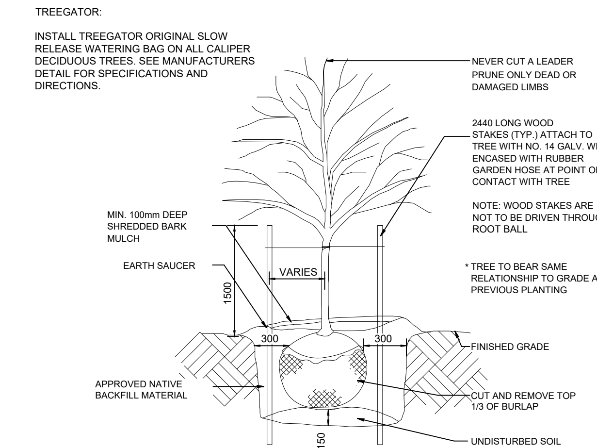
15 DECIDUOUS TREE PLANTING DETAIL NTS
