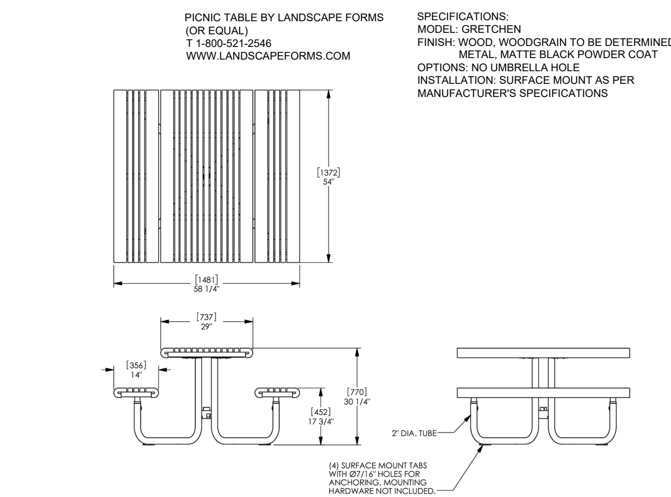
16 PICNIC TABLE DETAIL NTS
