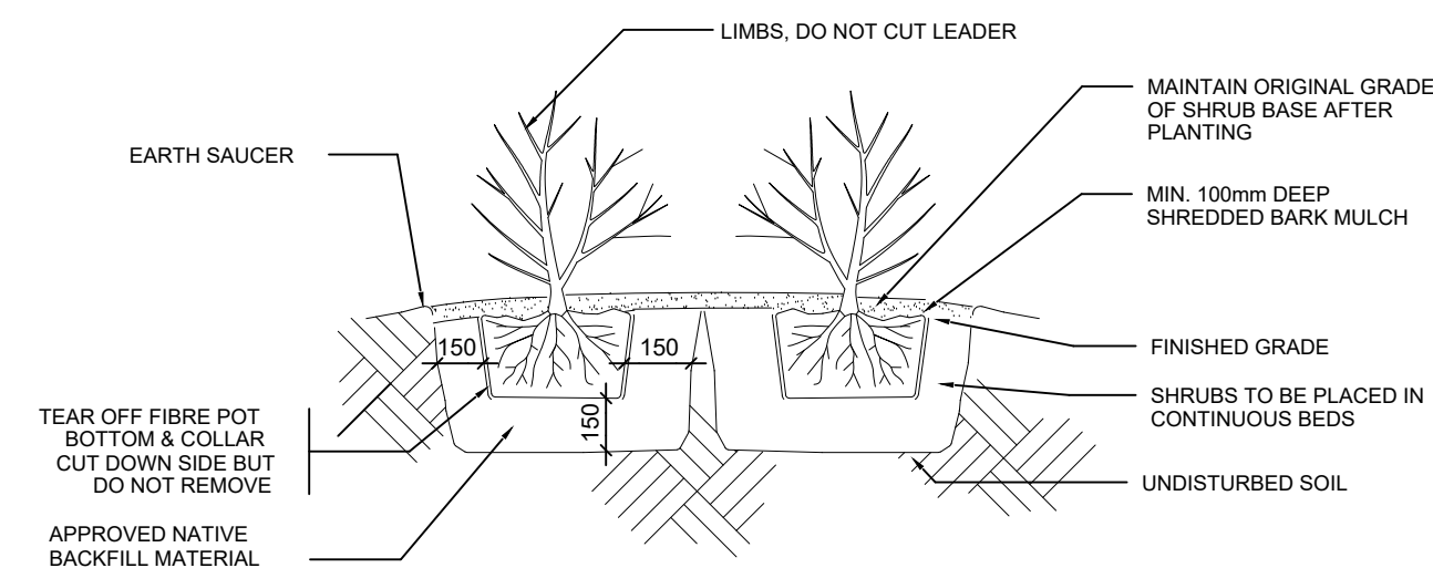
13 SHRUB PLANTING DETAIL NTS
