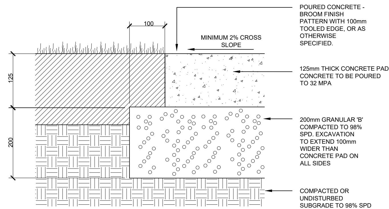
10 TYPICAL PIP CONCRETE PAD/SIDEWALK DETAIL NTS
