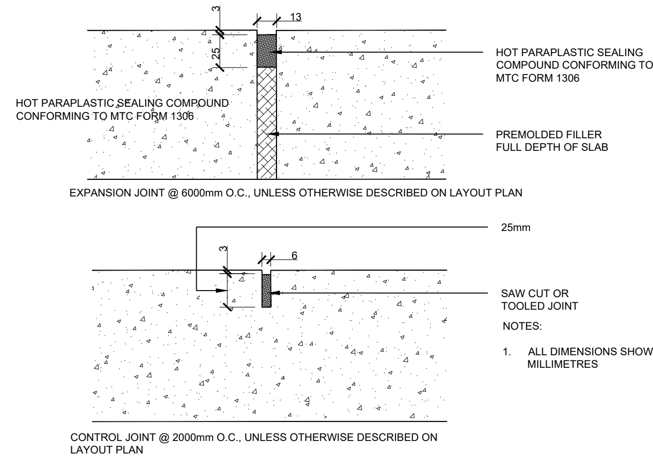
11 CONCRETE JOINT DETAILS NTS
