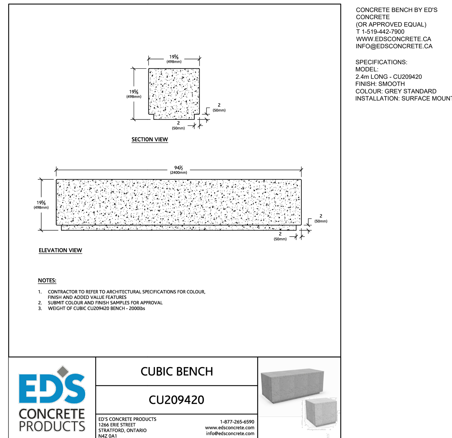
17 BENCH DETAIL NTS
