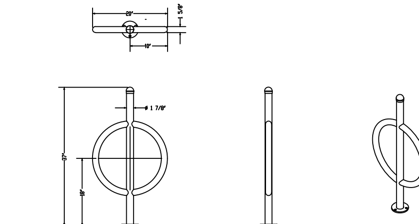
12 BIKE RACK DETAIL NTS
