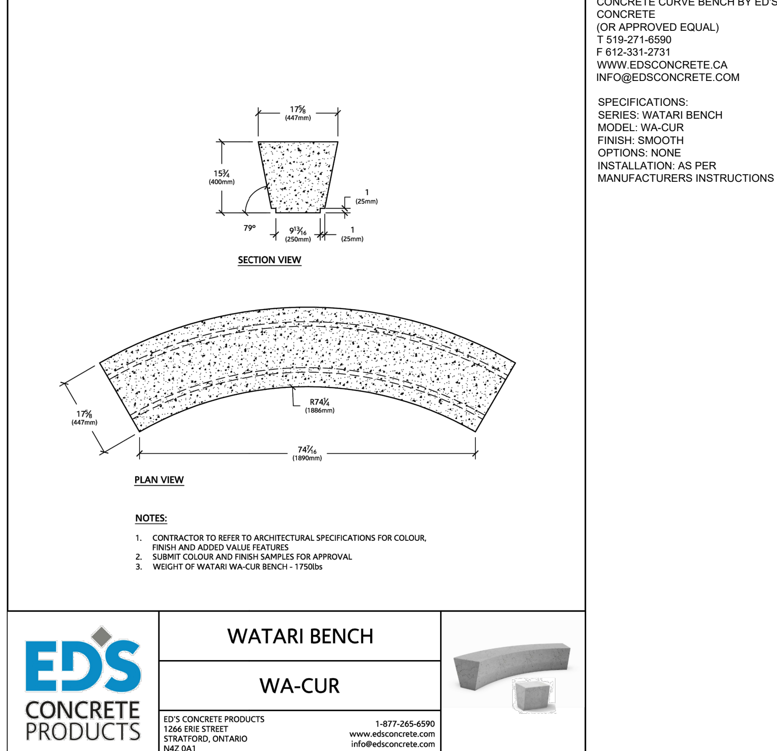
18 TYPICAL PRECAST CONCRETE CURVE SEAT WALL DETAIL NTS
