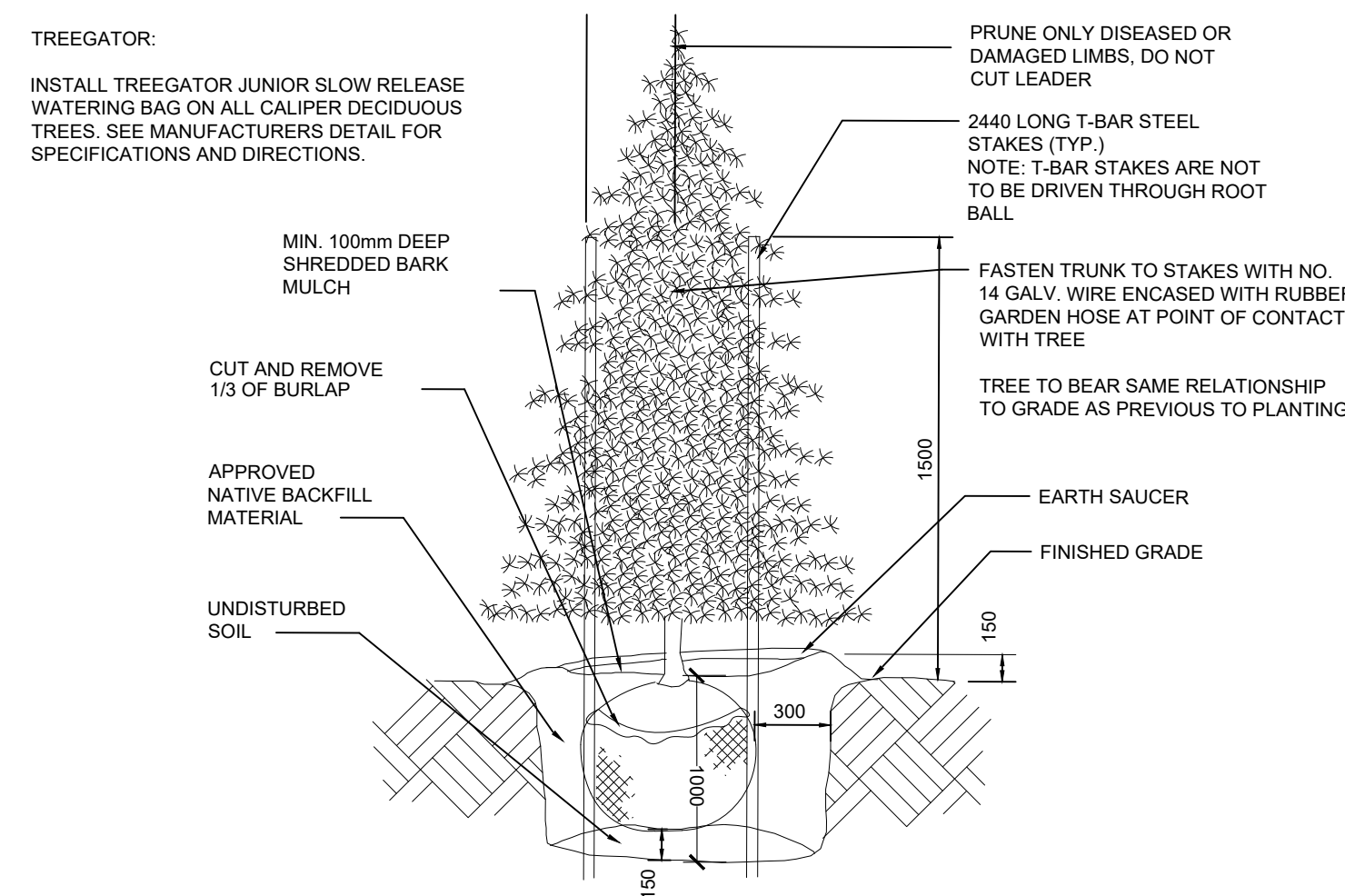
14 CONIFEROUS TREE PLANTING DETAIL NTS
