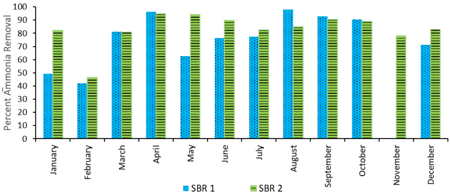
Figure 3: Per cent Ammonia Removal via Anammox, 2025
