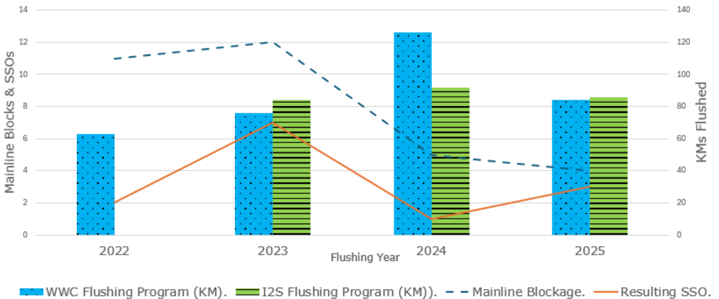
Figure 7: CCTV and Flushing Program vs. Mainline Blockage Response
