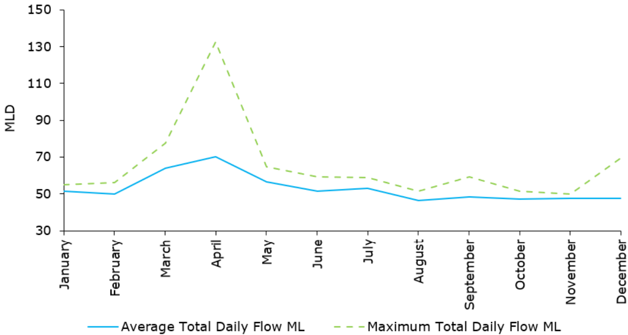
Figure 1: 2025 Average Daily Flow and Maximum Daily Flow
