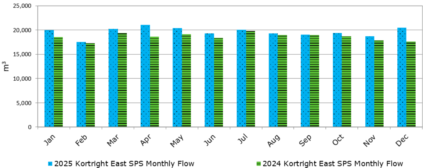
Figure 4: 2024 vs. 2025 Monthly Flow for Kortright East SPS
