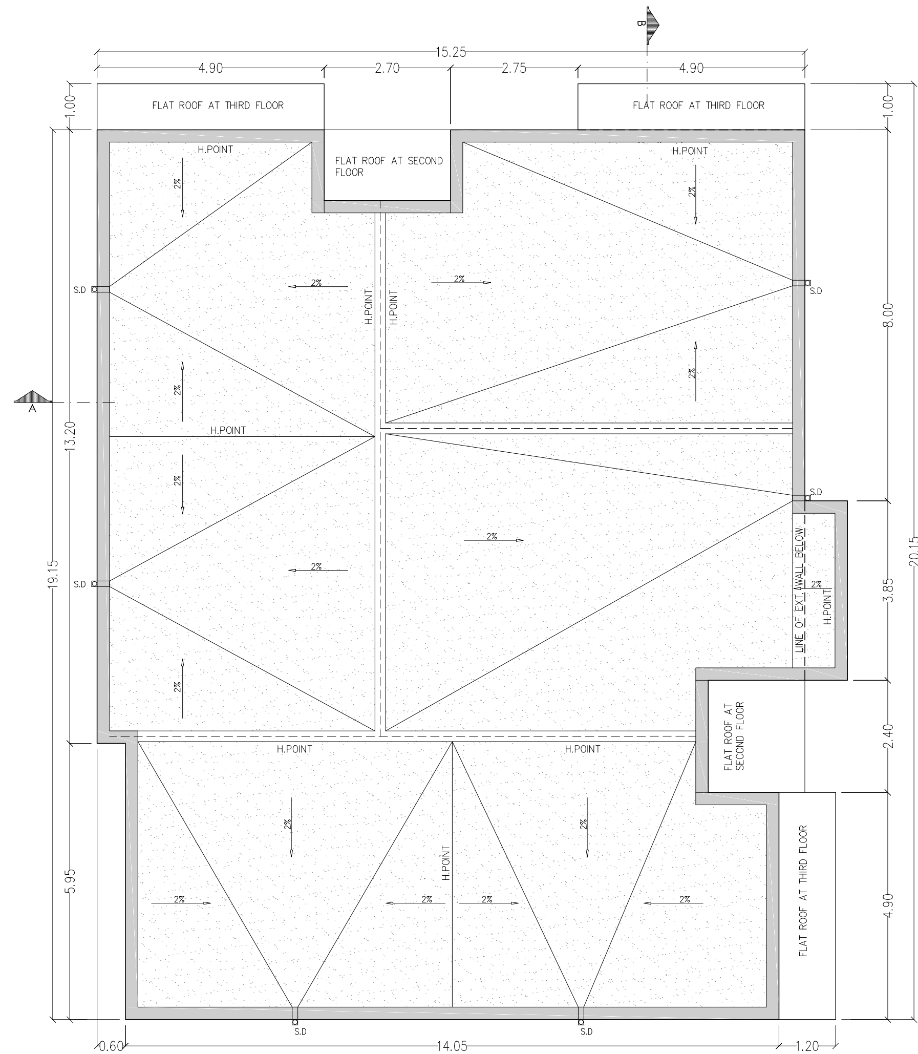
ROOF PLAN
