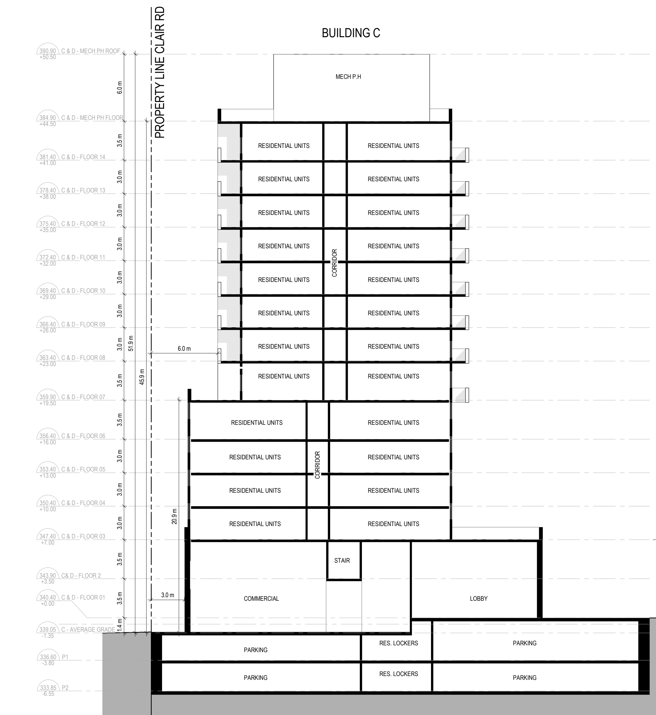
2 Section Building C & A A 401 1:200
