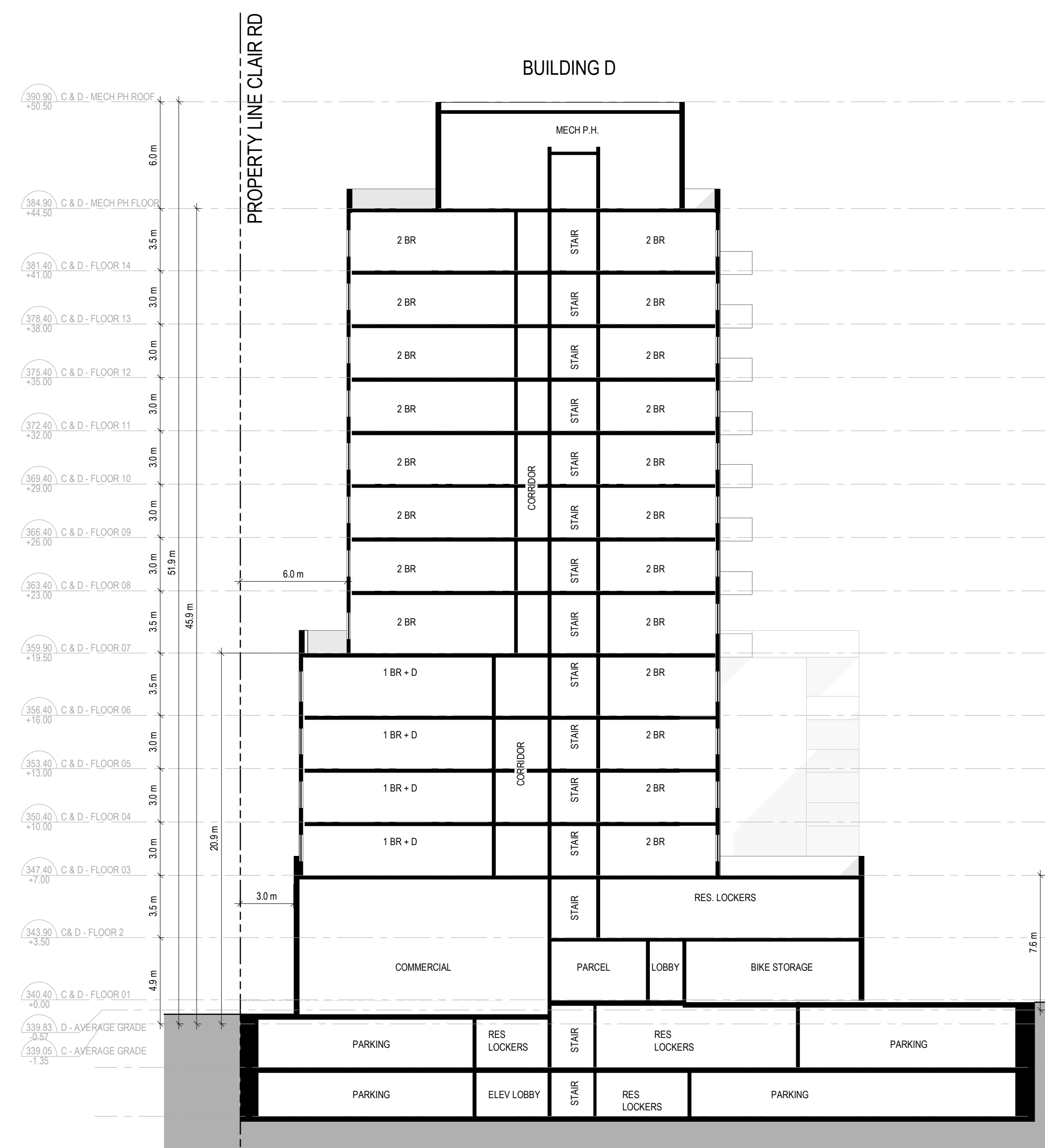
1 Section Building B & D A 401 1:200
