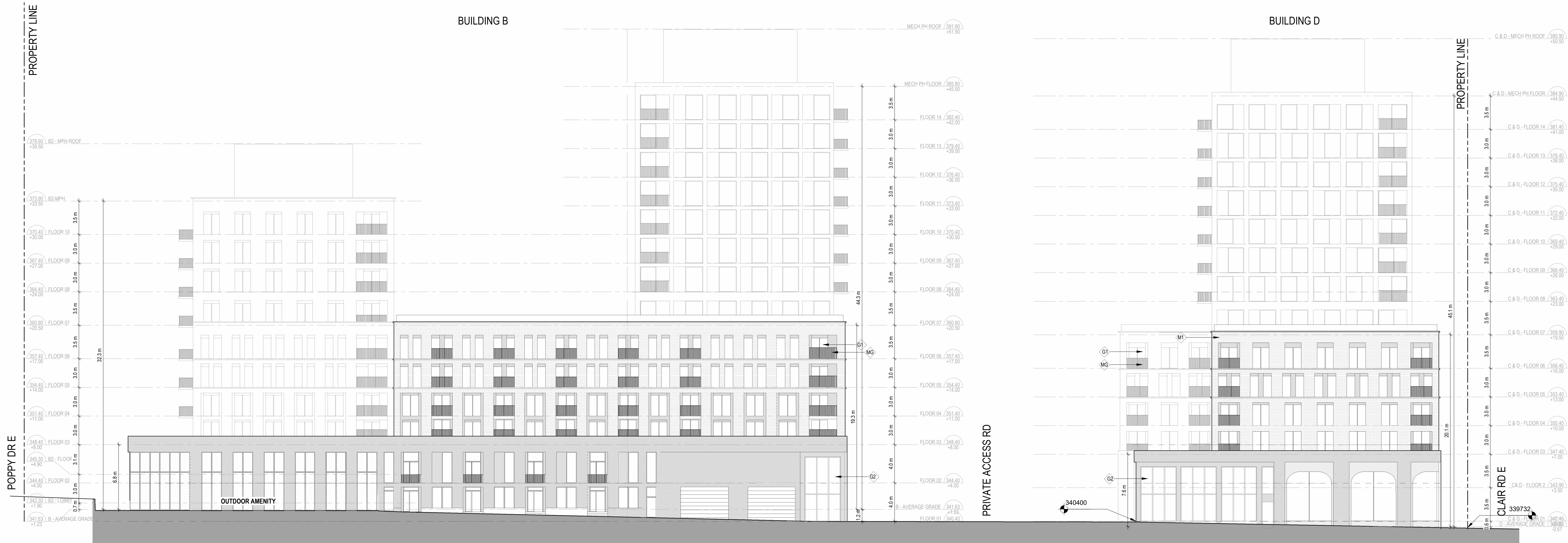
1 ELEVATION - BUILDING B & D EAST A 304/ 1:200
