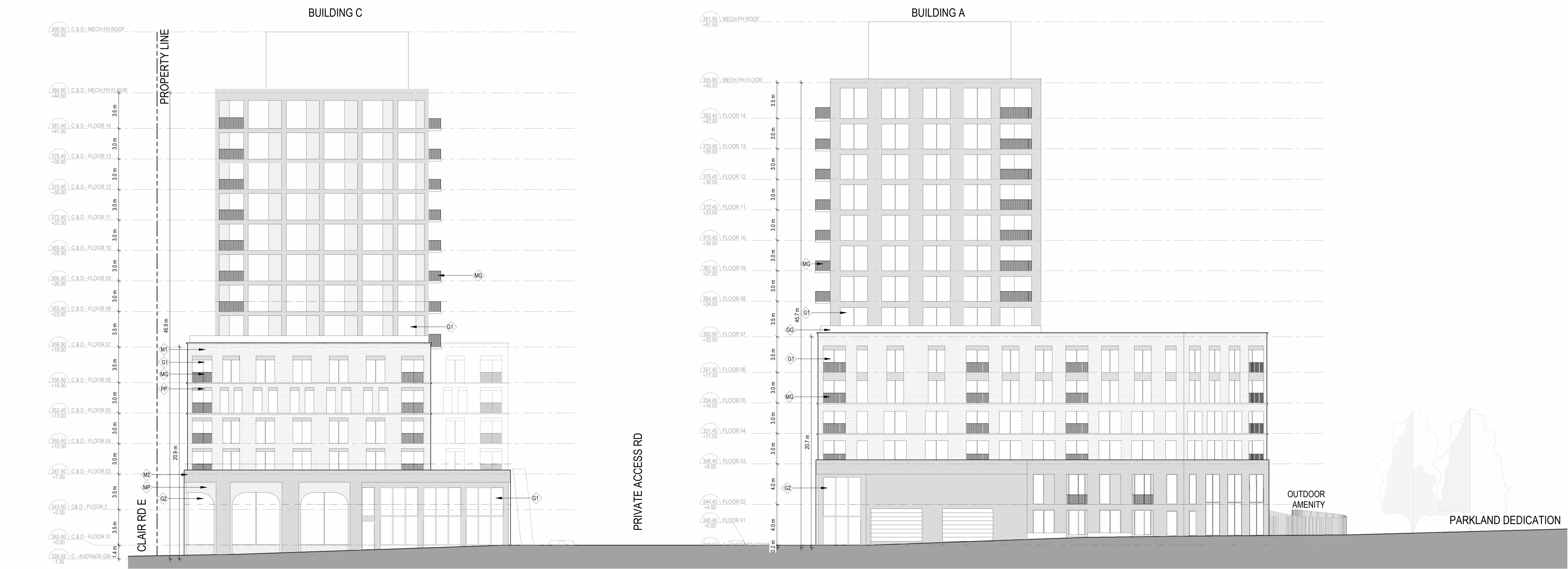
2 ELEVATION - BUILDING C & A WEST A 304/ 1:200
