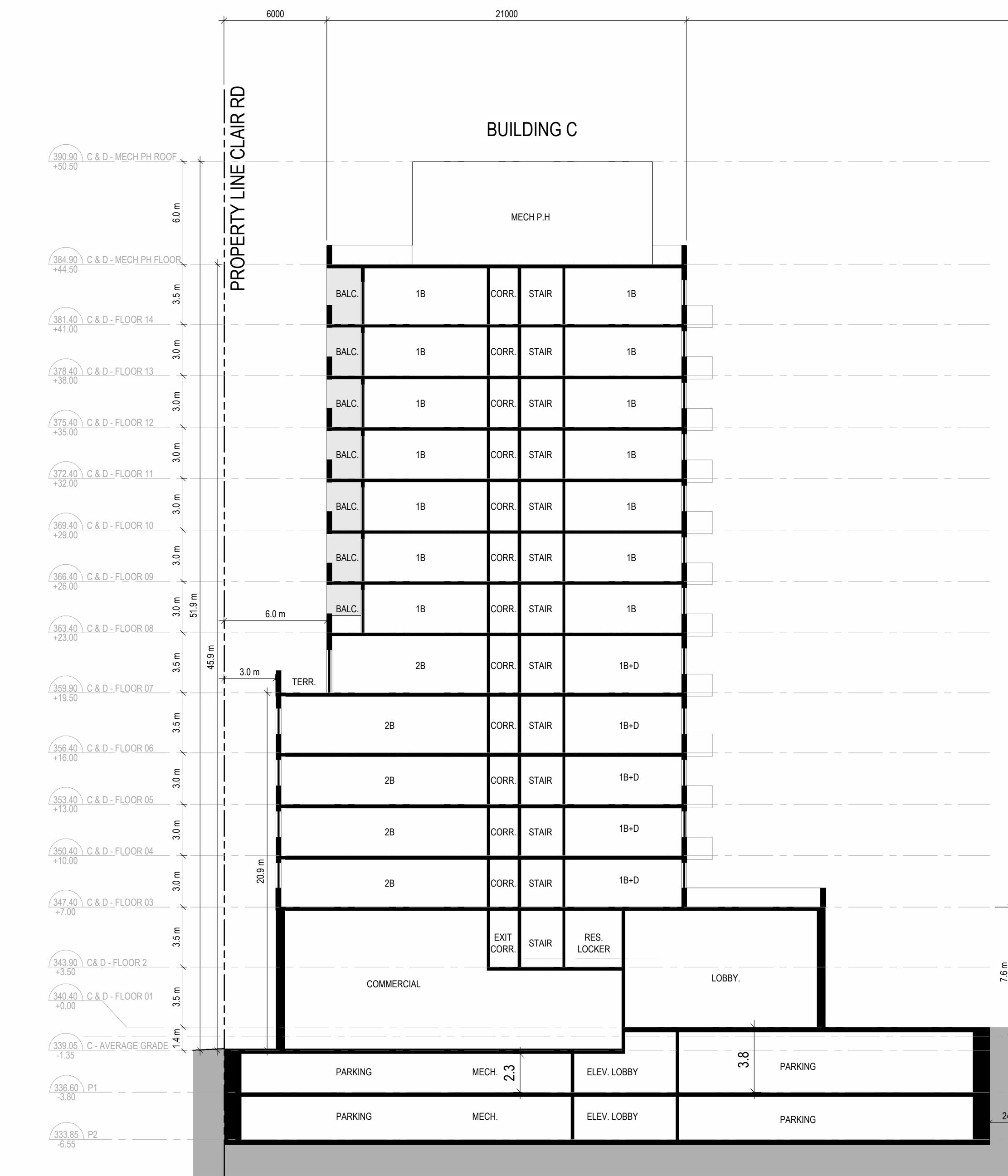
2 Section Building C & A A 401 1:200
