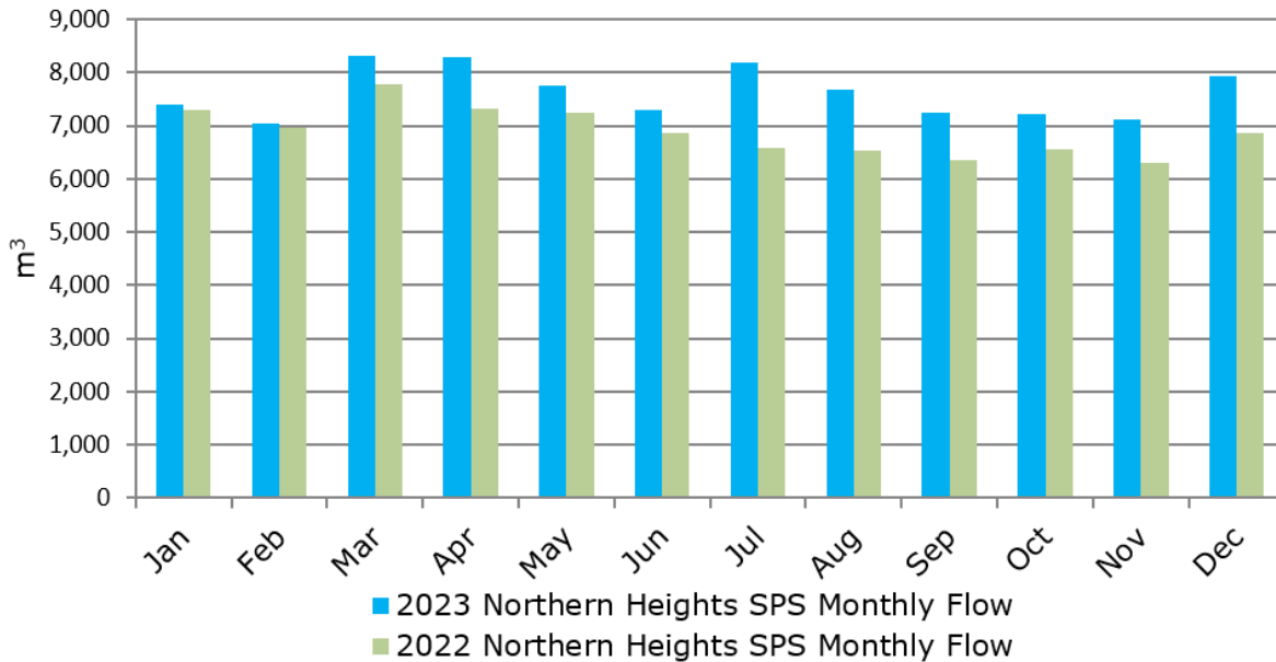
Figure 5: 2022 vs. 2023 Monthly Flow for Northern Heights SPS
