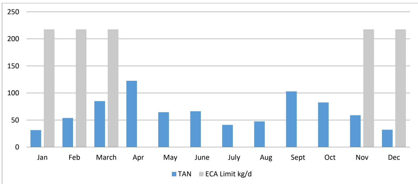
Figure 5 – 2023 Total Ammonia Nitrogen Loading
