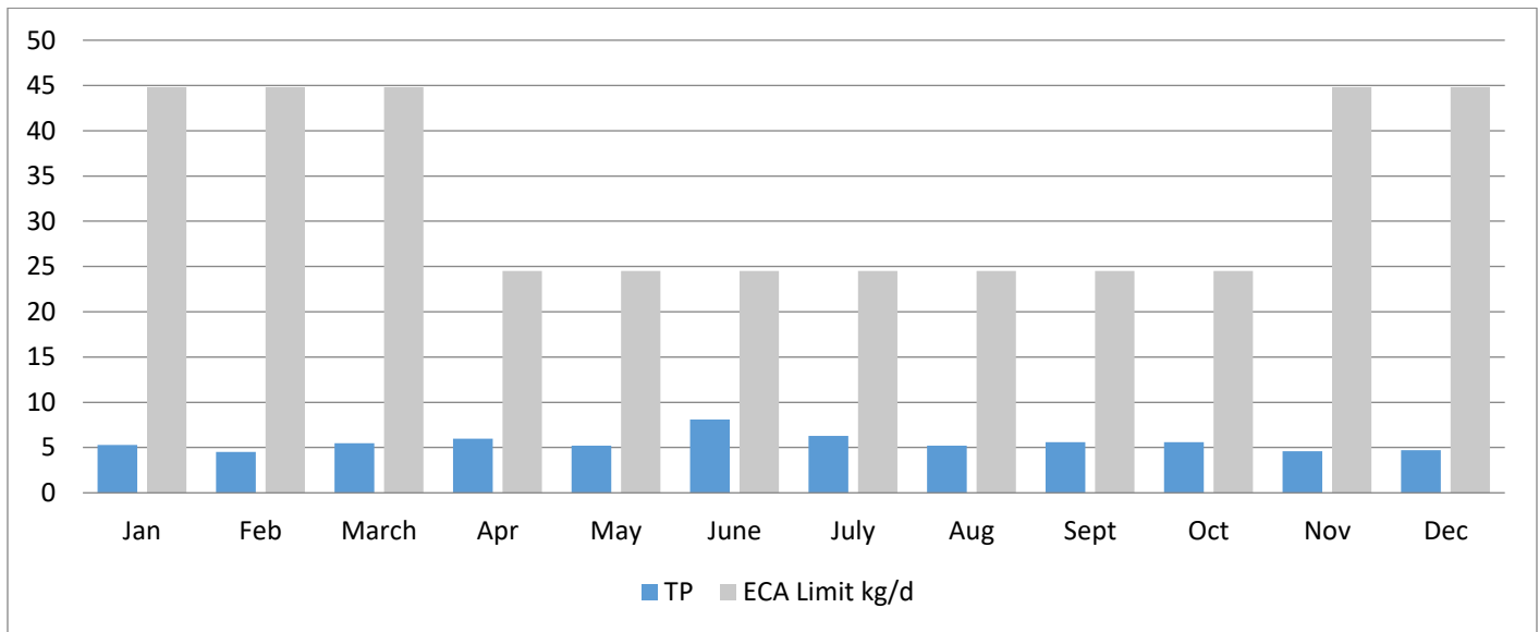
Figure 4 – 2023 Total Phosphorus Loading
