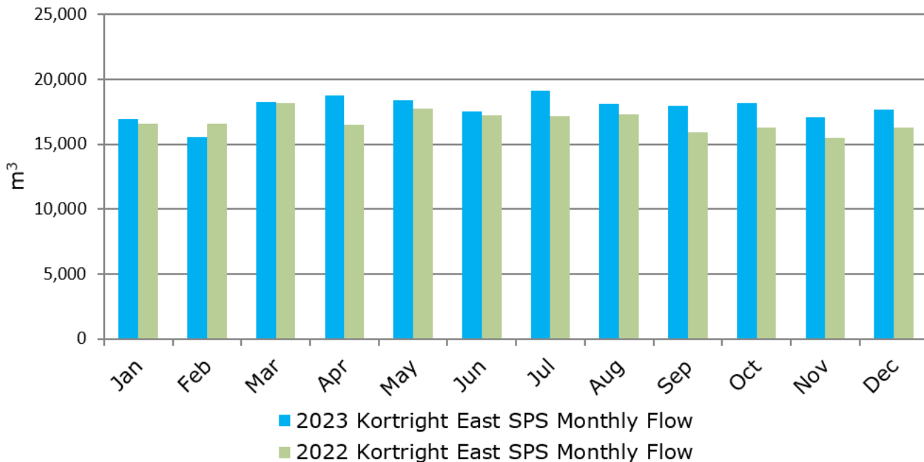
Figure 4: 2022 vs. 2023 Monthly Flow for Kortright East SPS
