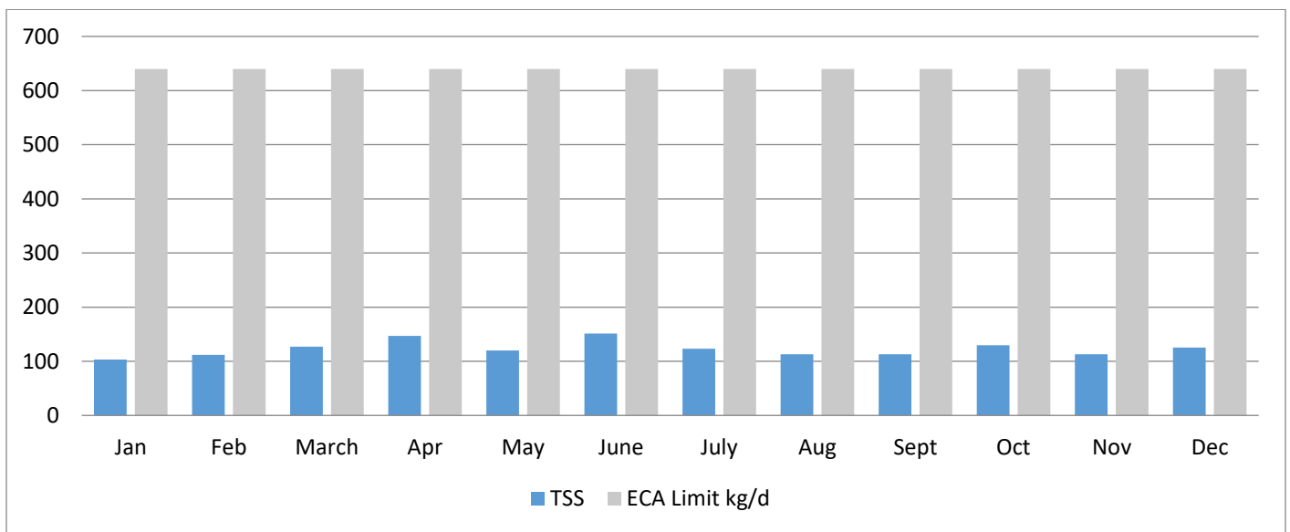
Figure 3 – 2023 Total Suspended Solids Loading
