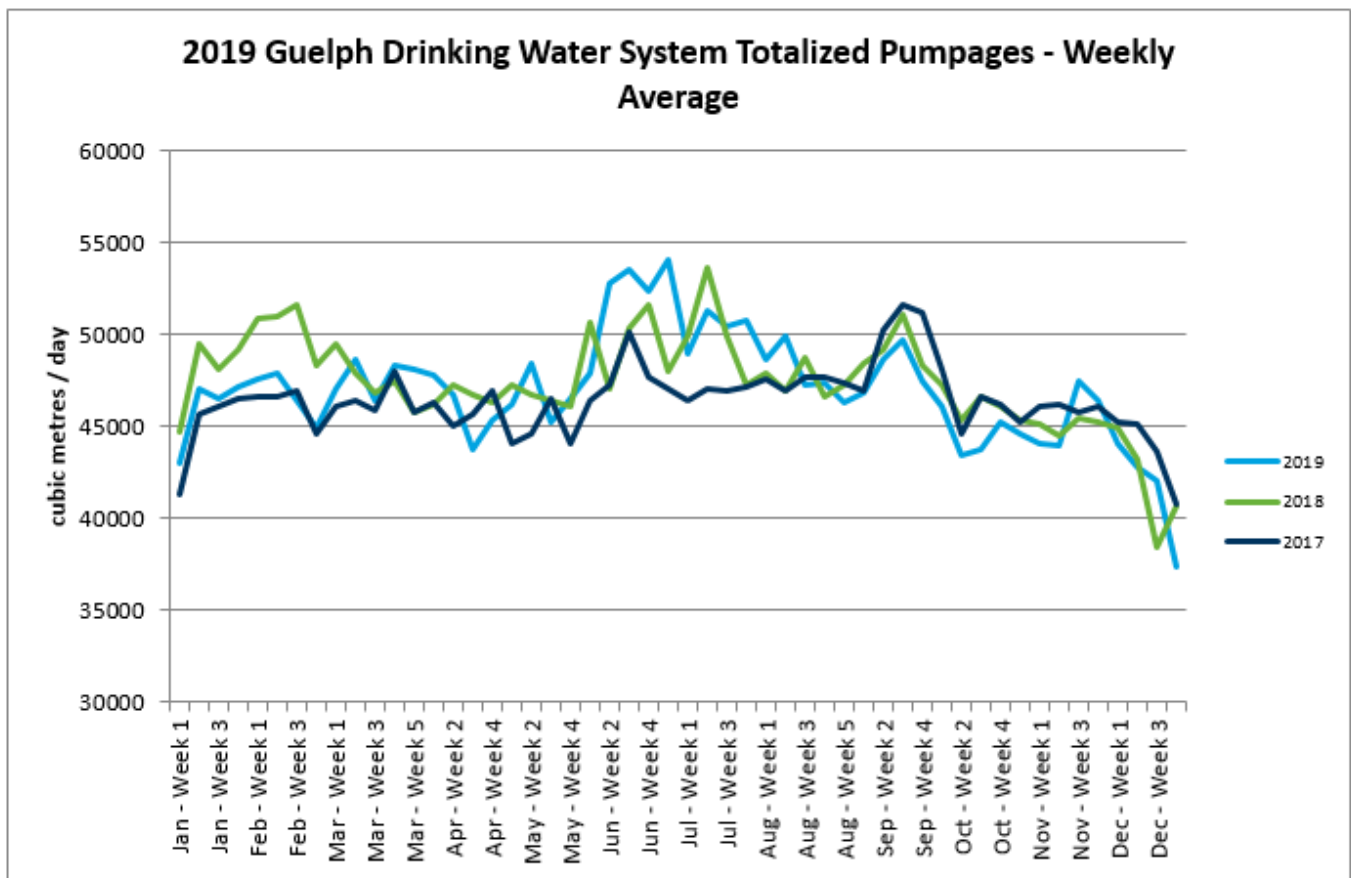
Figure 3: Totalized Pumpages, 2019
